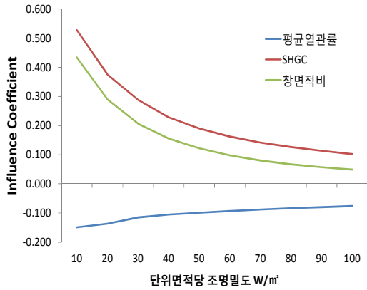
Fig 5 Influence Coefficients on the cooling energy demand (Daegu)
