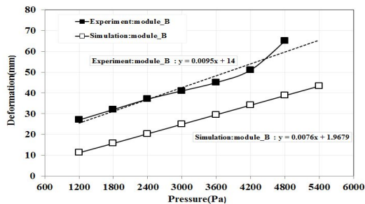
Fig. 3-6 The Deformation of PV Module (Module_B)
