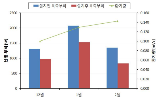
Fig. 5 Comparison of installation using SECOS-N 1
