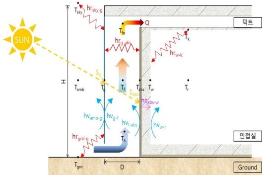
Fig. 3 Analysis of SECOS-N
