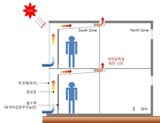
Fig. 2 Concept of system
