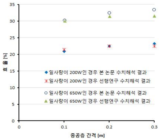
Fig. 4 Comparison of Simulation results
