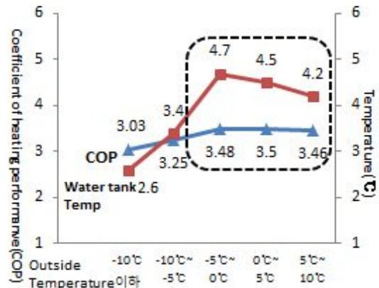
Fig. 5 COP graph according to outside temperature
